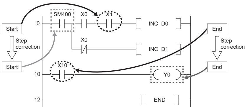
Program example
